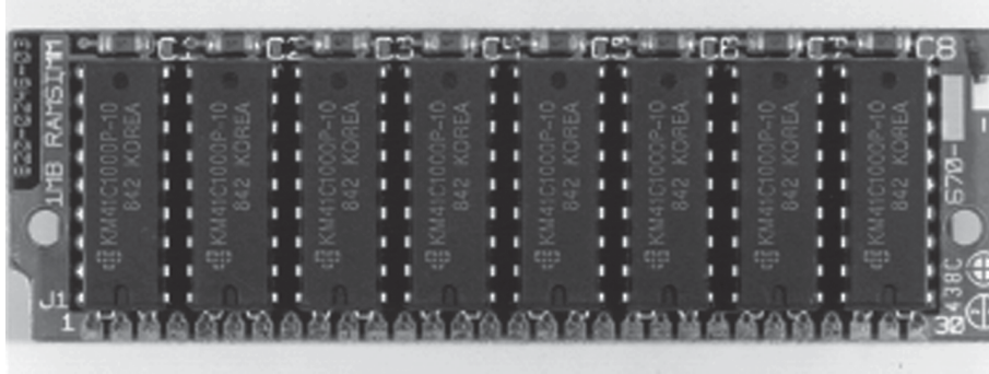
FIGURE 5.13.4 A 1 MB SIMM, built in 1986, using 1 Mbit chips. This SIMM sold for about $5/MB in 1997. As of 2006, most main memory is packed in DIMMs similar to this, though using much higher-density memory chips (1 Gbit).
