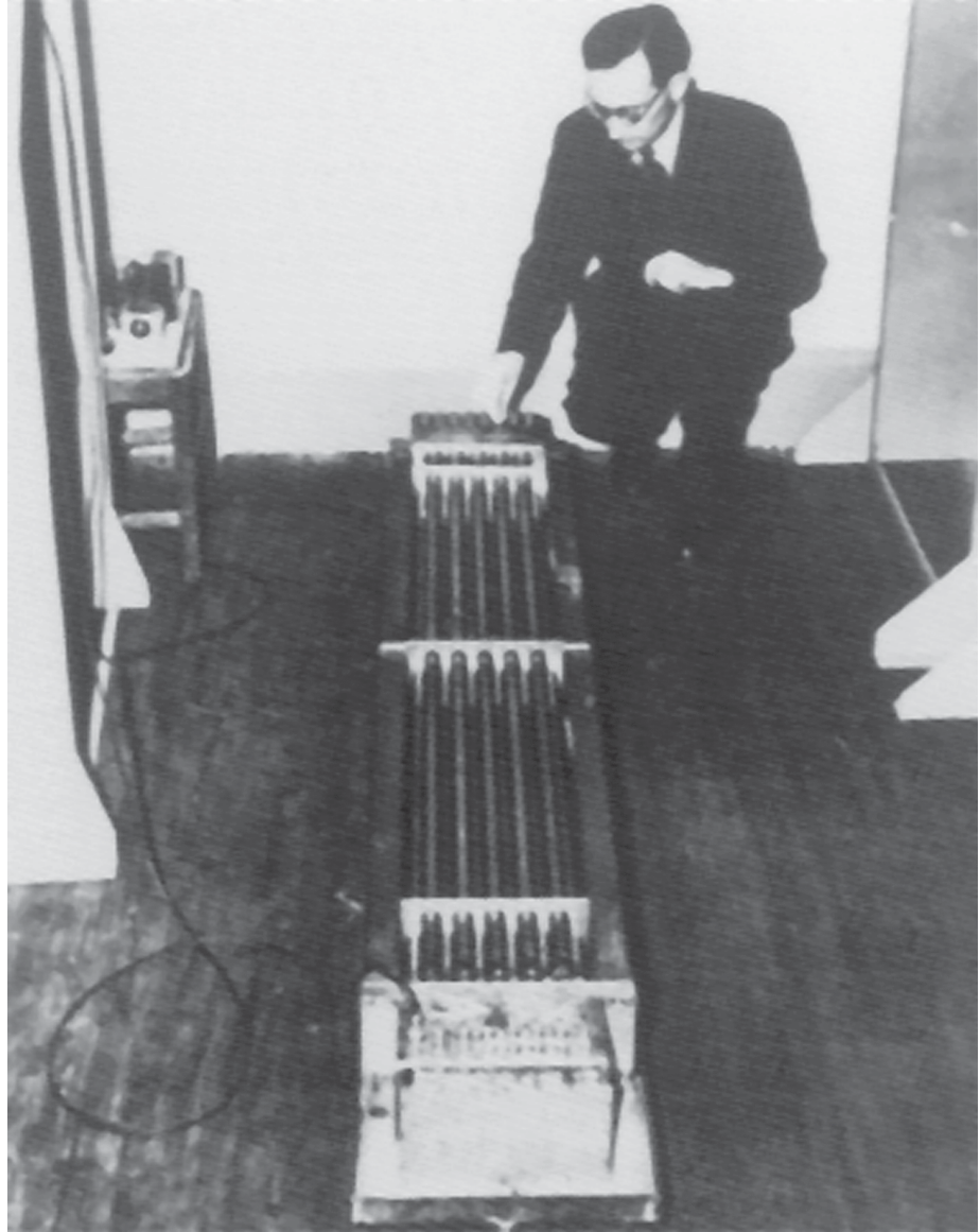
FIGURE 5.13.1 The mercury delay lines in the EDSAC. This technology made it possible to build the first stored-program computer. The young engineer in this photograph is none other than Maurice Wilkes, the lead architect of the EDSAC.
