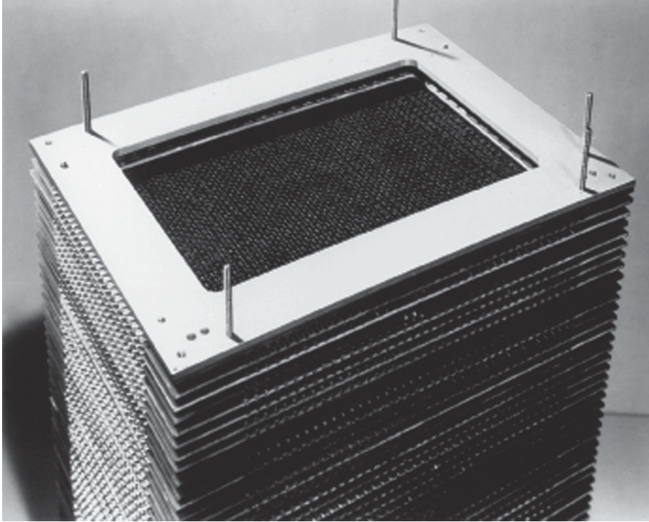
FIGURE 5.13.2 A core memory plane from the Whirlwind containing 256 cores arranged in a 16 x 16 array. Core memory was invented for the Whirlwind, which was used for air defense problems, and is now on display at the Smithsonian. (Incidentally, Ken Olsen, the founder of Digital and its president for 20 years, built the computer that tested these core memories; it was his first computer.)
